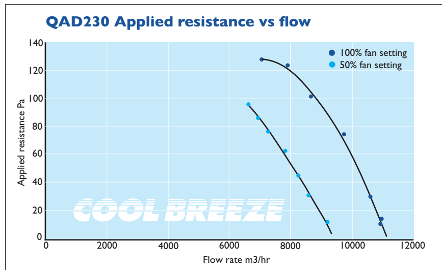
Powerflow fan with 'golf ball' dimpled blades
