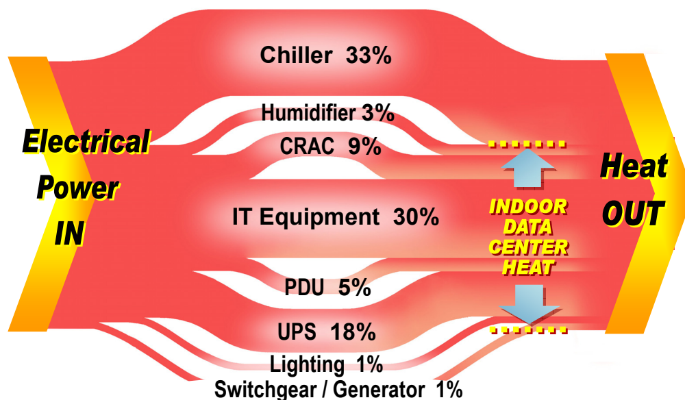
Figure 2 – Power flow in a typical 2N data center
