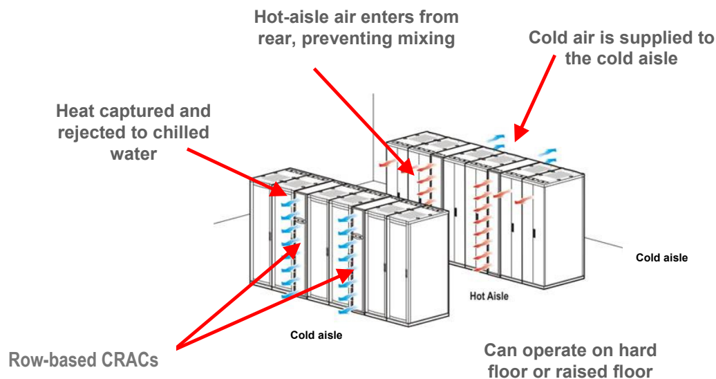
Figure 6 – Cooling using row-based CRACs with shorter air flow paths
