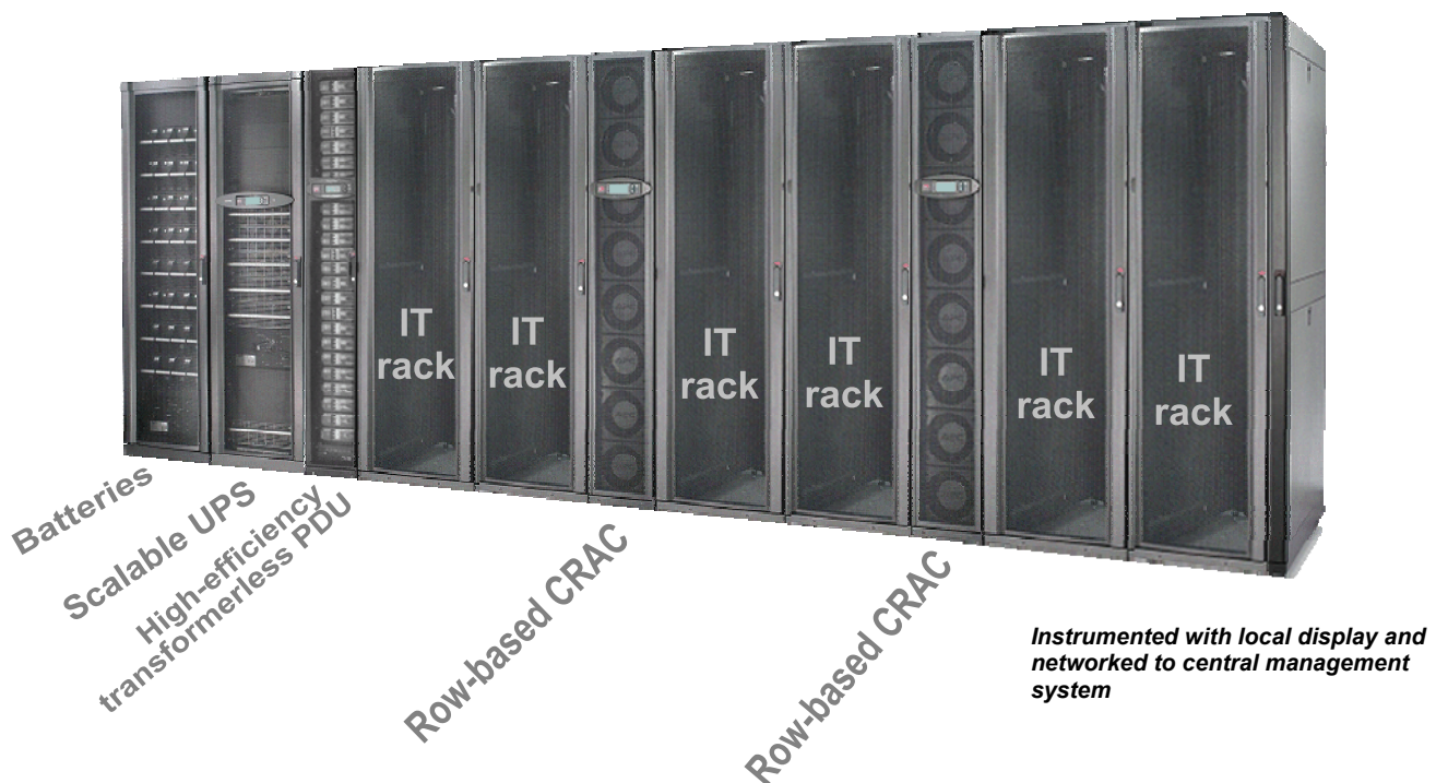
Figure 3 – High-efficiency integrated data center system
