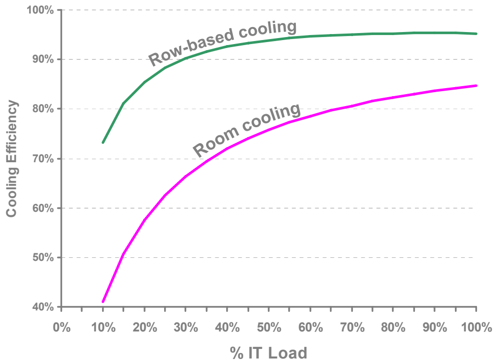
Figure 7 – Computer room air conditioner efficiency curves comparing row-based cooling to traditional room cooling
