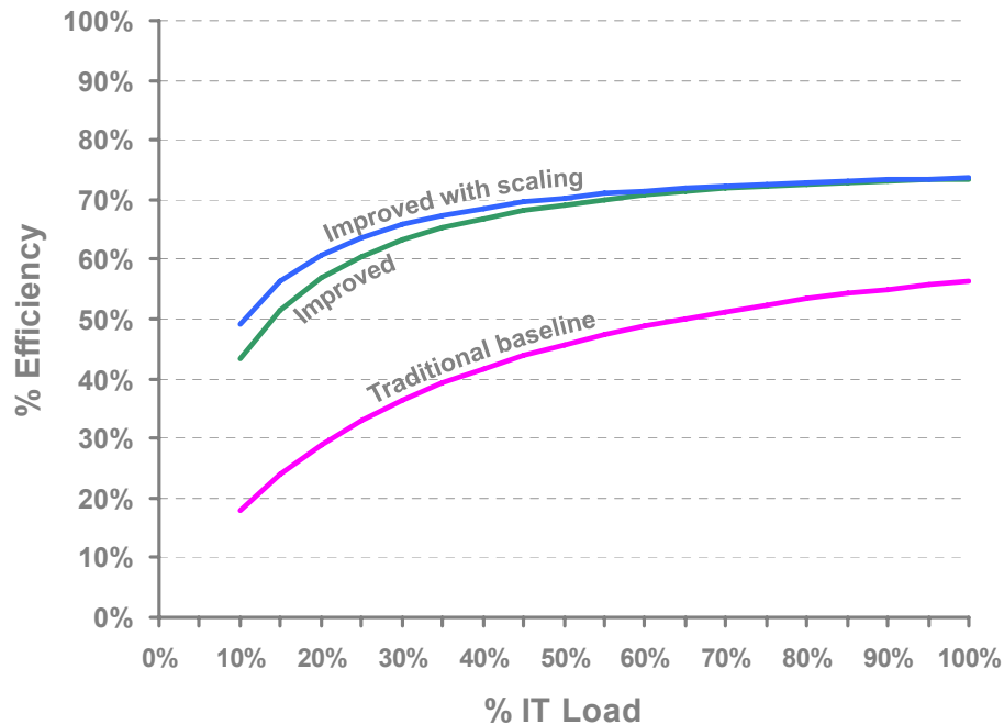
11b – Single power path, N air handlers
