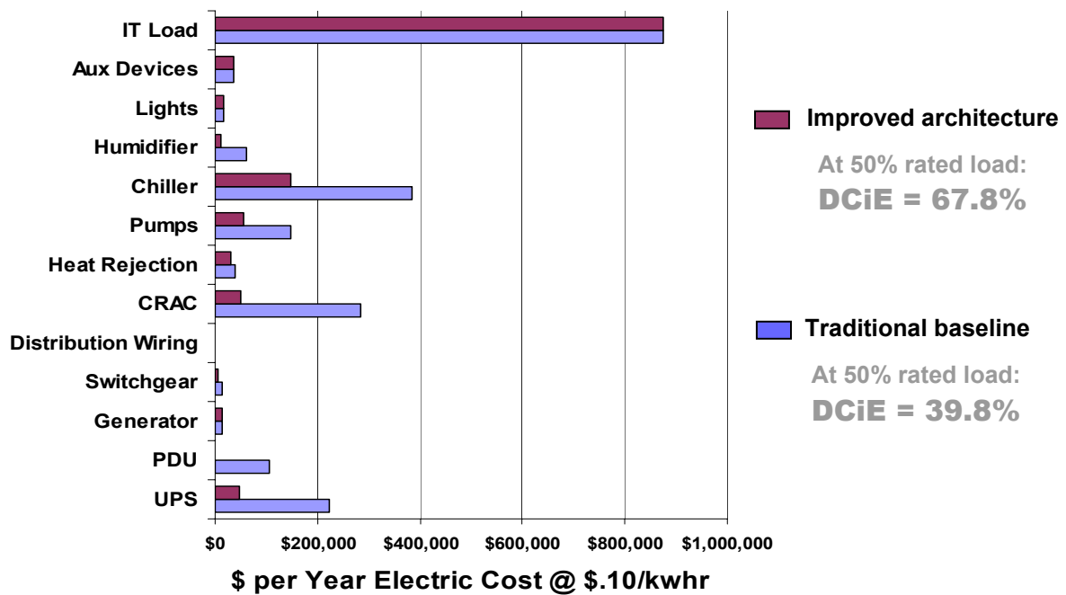
Figure 4 – Cost savings of improved architecture broken down by data center subsystem
